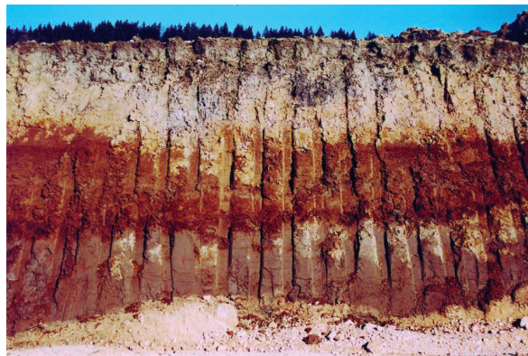
Figure 2: 7-metres-deep profile in the Grosuplje area. The bedrock is built by the Upper Triassic hauptdolomit.
