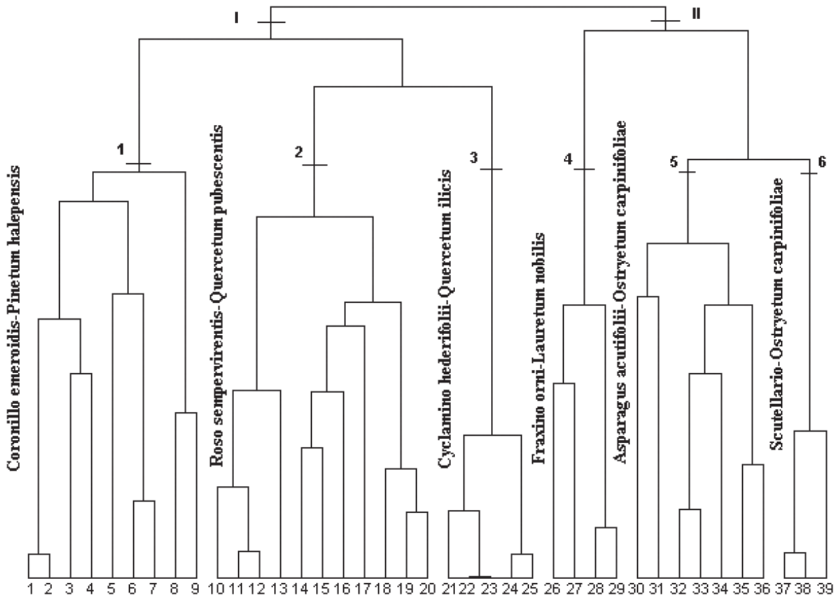
Figure 3: Dendrogram and classification of the forest relevés.
