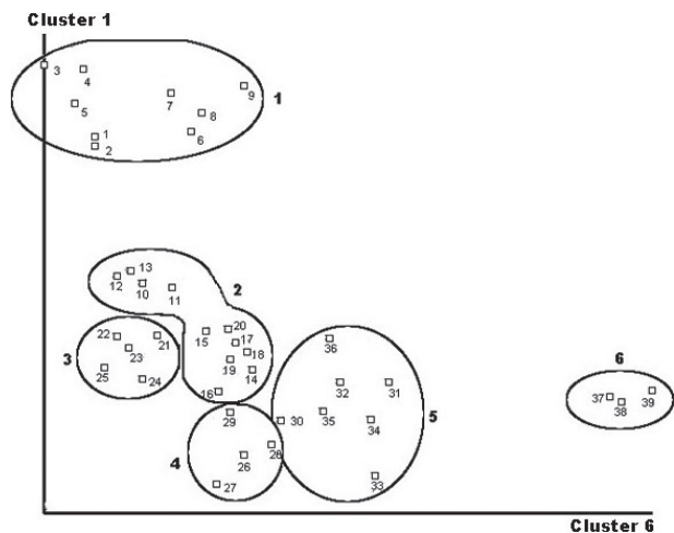
Figure 4: Ordination of the forest associations on the basis of the cluster 1 and 6 fuzzy sets.
