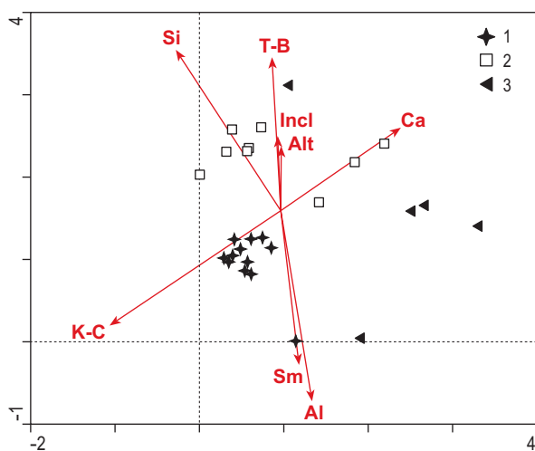
Figure 5: Diagram of the relevés classified within the classes Koelerio-Corynephoretea (1), Thero-Brachypodietea (2) and Stellarietea mediae (3) with explanatory variables passively projected onto the ordination space. For the abbreviations of explanatory variables see Figure 4.
