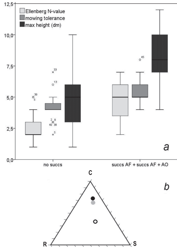
Figure 7: Distribution of plant traits among species that successfully colonised restoration sites (succs AF + succs AF + AO) and those who failed to do so (no succs) (a). The successful and unsuccessful group differed significantly in their mean trait values: Ellenberg N, mowing tolerance, max height (Mann-Whitney- U test, p \leq 0.001 ). Strategy triangle plot (b) of species groups (black dot: succs AF+AO, grey dot: succs AF, black ring: no succs). no succs: unsuccessful colonisers, succs AF + succs AF+AO: successful colonisers of the arable field and of the apple orchard, C: competition, R: disturbance, S: stress.
