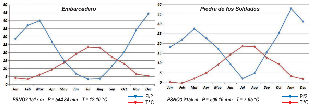
Figure 2a: Climatic diagram of the study site (meteorological station: “Embarcadero” PSN02, 1517 m).
