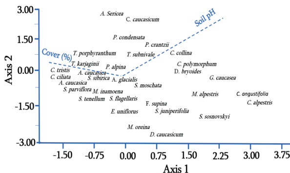
Figure 7: CCA ordination diagram of plant species composition between two study sites (Gudauri and Kazbegi) in alpine-nival ecotone (3000 m a.s.l.) in the Central Caucasus; plant cover (%) and soil pH are used as environmental variables (Species full names are given in Table 1).
