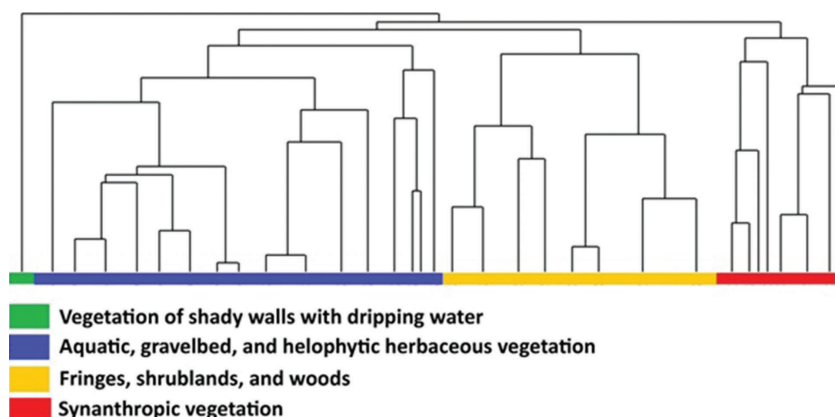
Figure 2: Dendrogram resulting from the UPGMA cluster analysis. The colored bars correspond to the relevés included in each cluster. Slika 2: Dendrogram UPGMA klastrske analize. Obarvane črte predstavljajo popise, ki so vključeni v vsakega od klastrov.
