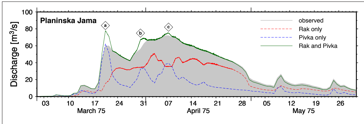
Fig. 14: Observed (grey) and modelled (blue, red, green, see legend) discharge data at the resurgence of Planinska Jama for the period Mar-May 1975. The time is given in days starting on 1 st March 1975.
