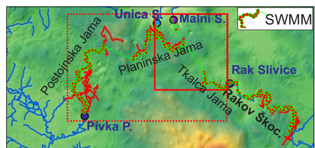
Fig. 13: View of the aquifer system comprised between Cerkljško Polje, the Pivka Valley and Planinsko Polje with the network of conduits built in SWMM. The solid rectangle marks the domain modelled in these paper. The dotted rectangle marks the domain including the flow of Pivka through Postojnska Jama and Pivka Branch.
