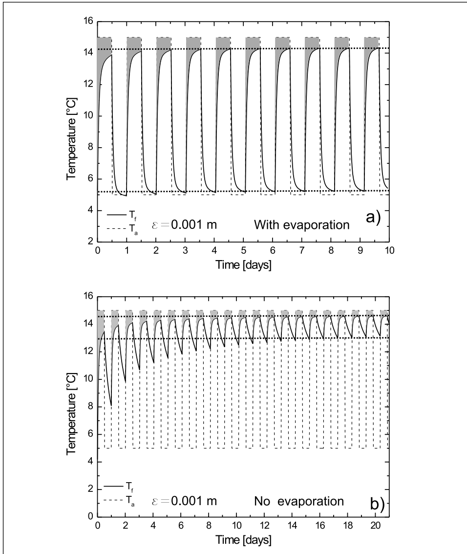
Fig. 7: Wall temperature for diurnal temperature variations of T_a in the cave. For simplicity an abrupt change between day temperature T_{day} and lower night temperature T_{night} is assumed. The initial temperature of the cave wall T_{fi} < T_{night} . a) Water accumulated at the surface by condensation during day time evaporates during night time. Rates of heating during the day and cooling during the night are almost equal. Average rates of condensation are high. b) Condensation during day time, but evaporation during the night is absent. Therefore the rate of cooling is only about 15% of the heating rate during daytime. A steady state with less average condensation is reached after several cycles. Note that the shaded areas give a measure of condensed water. The two parallel dotted lines present upper and lower temperatures at steady state.
