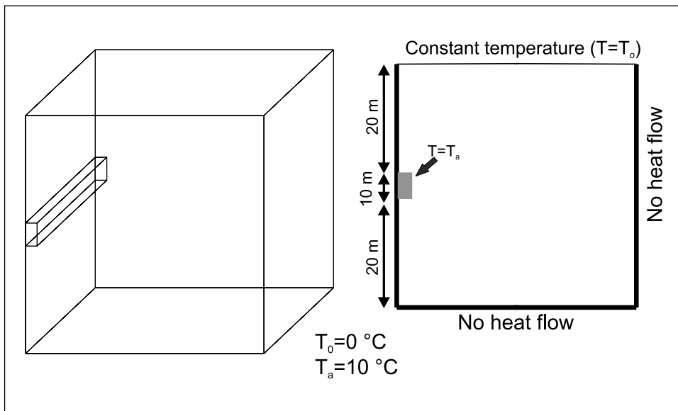
Fig. 10: Modeling domain of a rectangular conduit. Only the right half is shown, because of the mirror symmetry. The surface temperature is T=T_o . All other boundaries are impermeable for heat flow.
