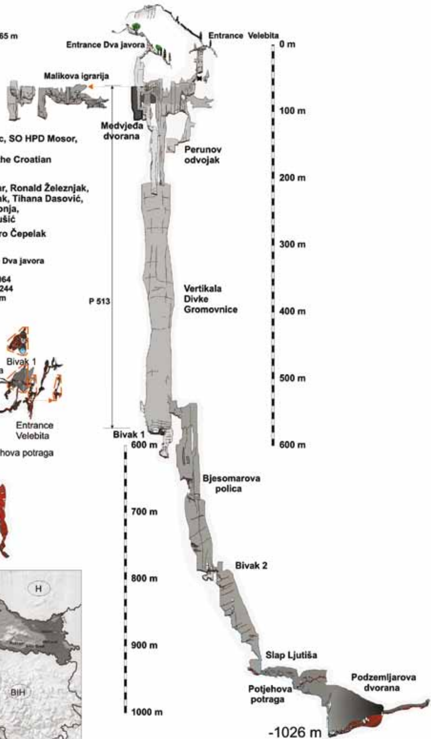
Fig. 1: Velebita Cave system. Insert: Location of the cave.
