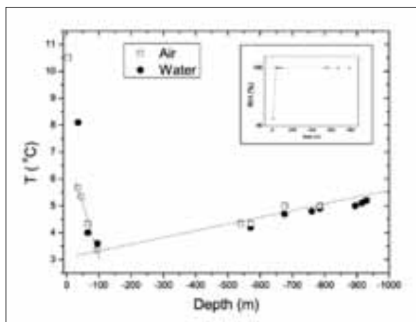
Fig. 2: Air and water temperature variation with the cave depth (5.-12.8.2007.). Dashed lines are two different linear regressions of air temperature between -30 and -100 m, and -100 and -800 m. Insert: Relative air humidity RH% as a function of the cave depth.
