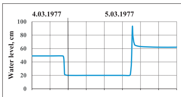
Figure 11: Diagram of the water level in the Izcrets Spring limnigraph during the interruption associated with the Vrancea earthquake in 1977 (after Petrov, 1983).
