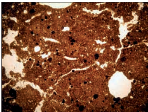
Fig. 10: Massive microstructure of horizon Bw in doline D17, with many sub-rounded channels (16x PPL).
