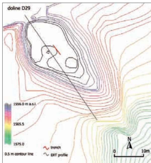
Fig. 4: Detailed topography of D29 (obtained by a field survey).
