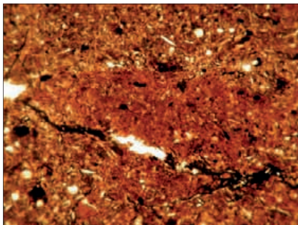
Fig. 15: Microstructure of horizon Bw1 with several channels in doline D29 (16x PPL).
