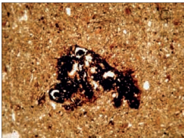
Fig. 13: Ameboidal Fe/Mn nodule in horizon Btg indicating poor soil drainage, doline D29 (40x PPL).
