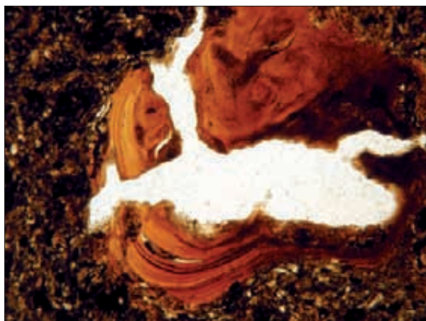
Fig. 14: Reddish pedorelict in horizon 2Bt2, doline D29 (100x PPL).
