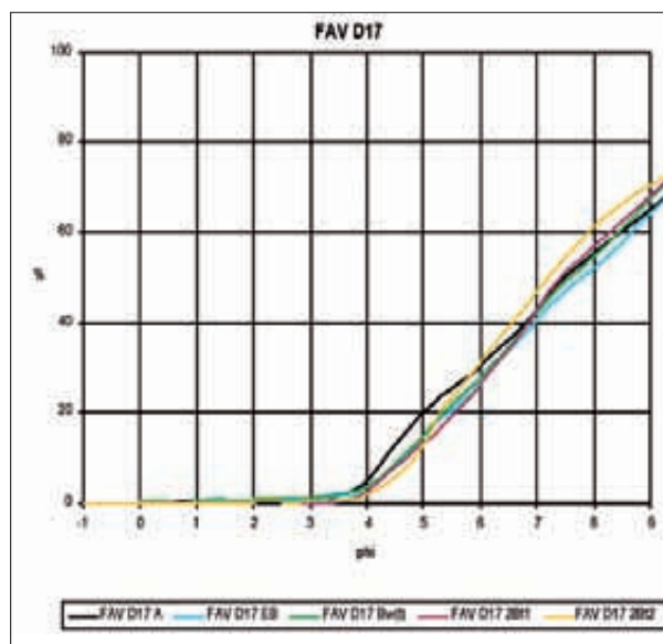
Fig. 8: Cumulative particle size curves of five samples of D17; \phi = -\log_2 (particle size in mm).
