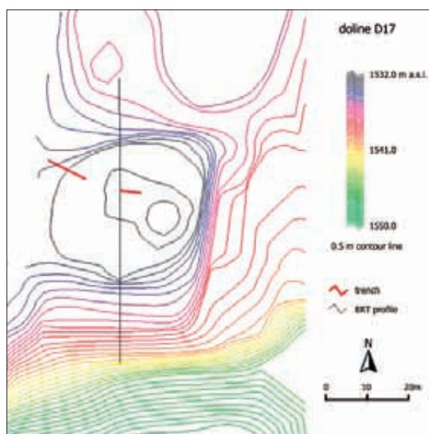
Fig. 3: Detailed topography of D17 (obtained by a field survey).
