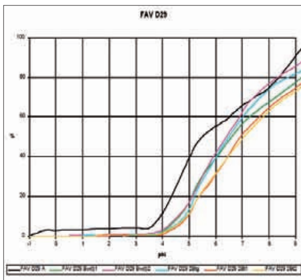
Fig. 9: Cumulative particle size curves of six samples of D29; \phi = -\log_2 (particle size in mm).
