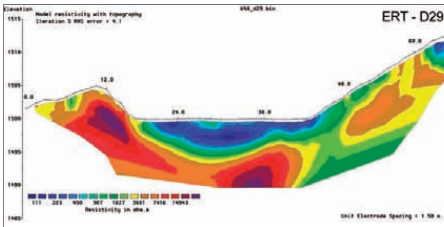
Fig. 6: Electric tomography profile of D29.
