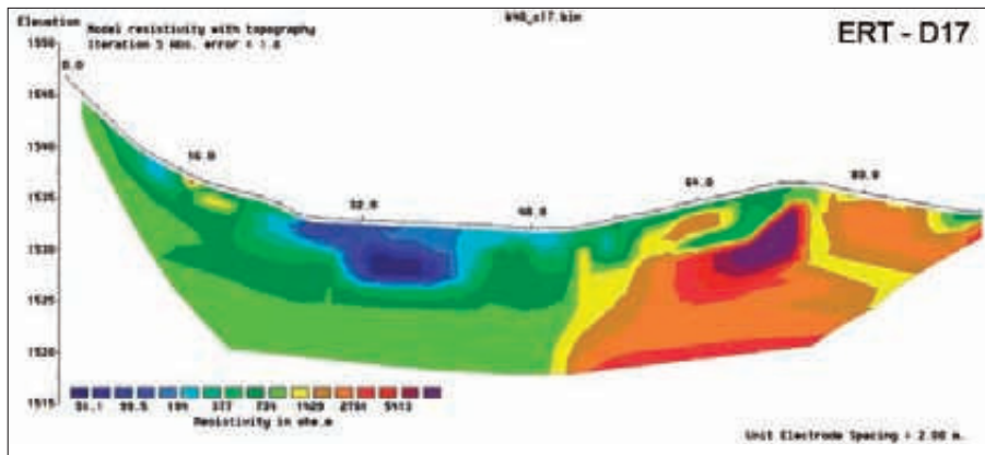
Fig. 5: Electric tomography profile of D17.
