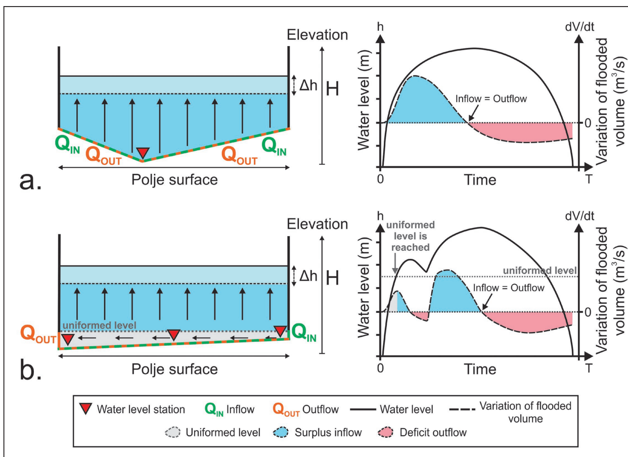
Figure 1: Flooding dynamics in a conceptual polje with measured water level and variation of flooded volume. (a) Situation when flooding is solely caused by a rise of the regional groundwater level. (b) Situation when flooding is caused by a combination of inflow provided by rivers and karst springs and rise of the regional groundwater level.
