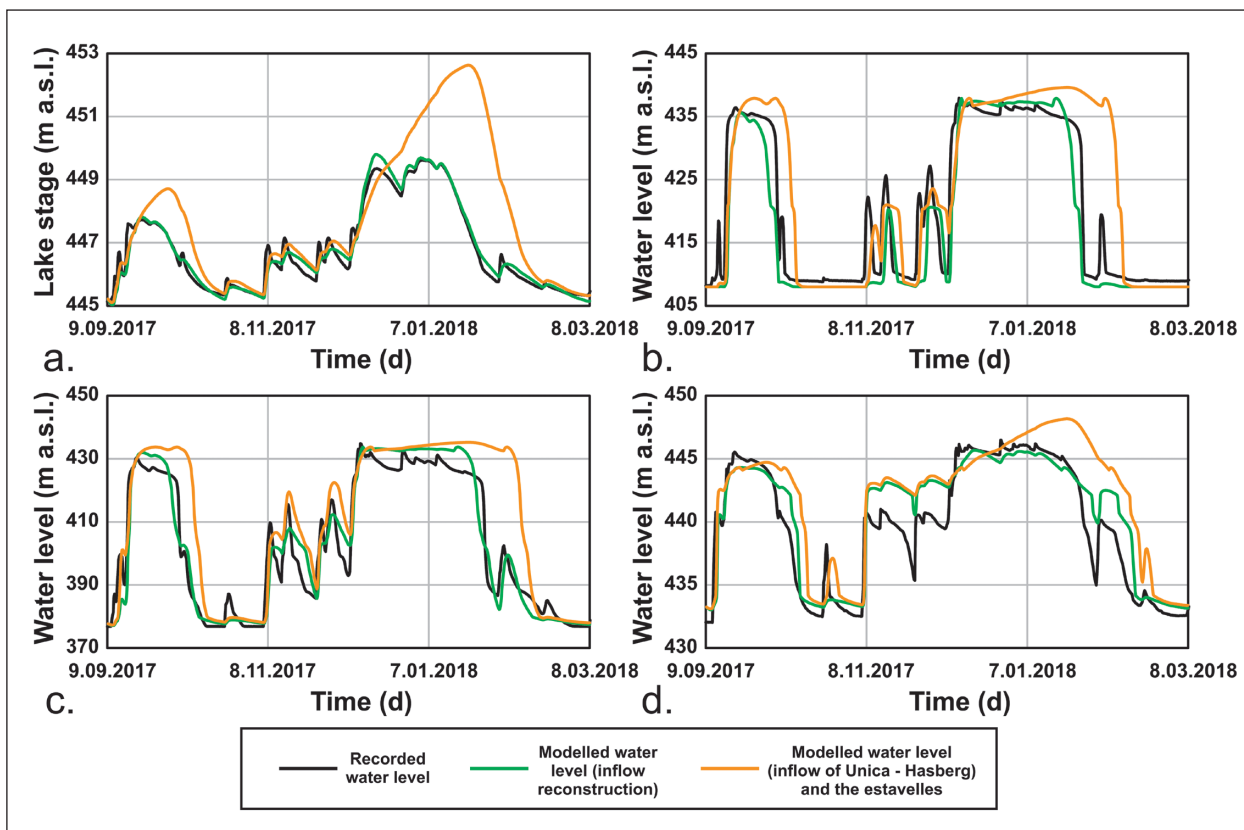
Figure 10: Measured and simulated water levels during the floods of September and December 2017 for (a) Planinsko Polje; (b) Najdena Jama; (c) Gradišnica; (d) Logarček.
