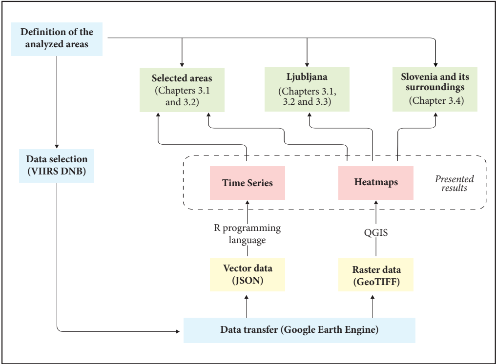
Figure 1: Analysis of Light Pollution in Slovenia flow chart.
